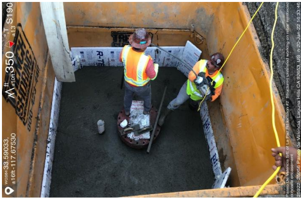
Reinforced Concrete Encasement at Paseo De Valencia Location
