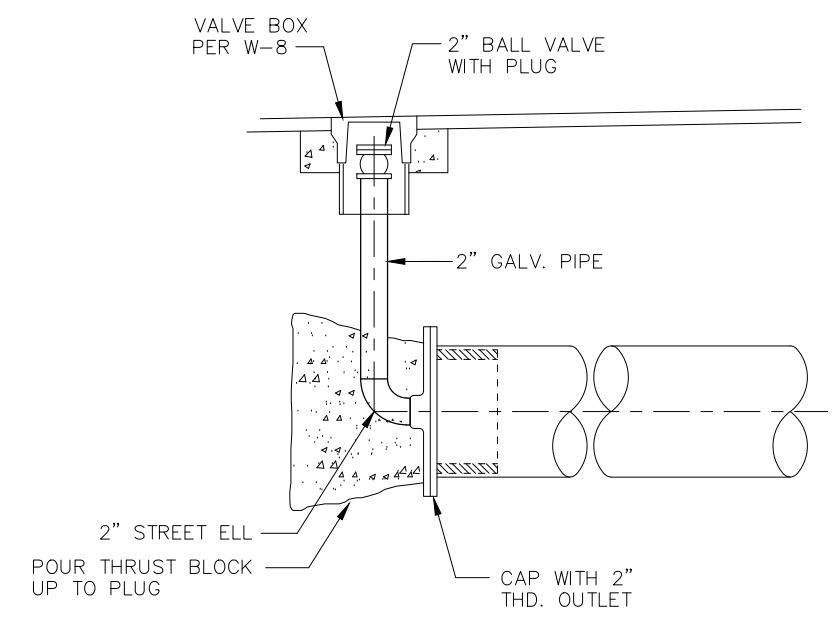
TEMPORARY PLUG & BLOWOFF
