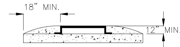
CONCRETE COLLAR DETAIL PLAN VIEW
