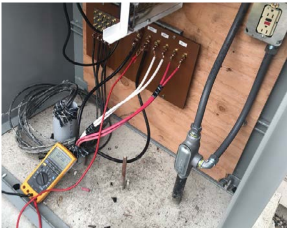
Testing of New Rectifier
