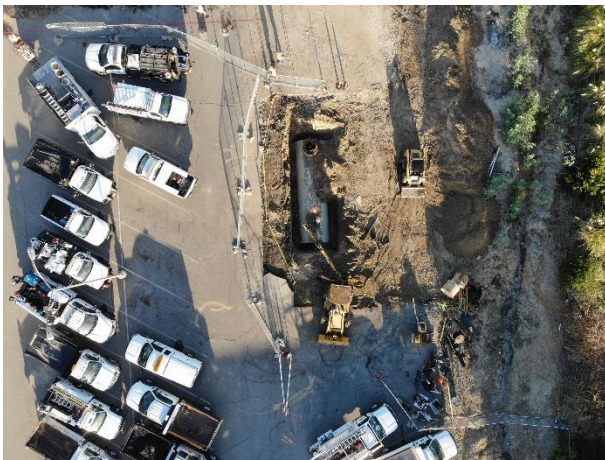
Removal of Existing Fuel Storage Tank
