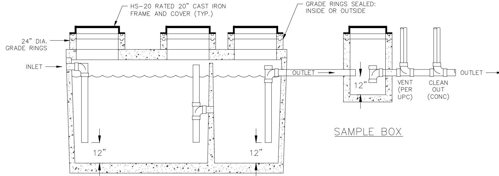
SIDE VIEW
