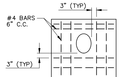
REINFORCING STEEL PATTERN
