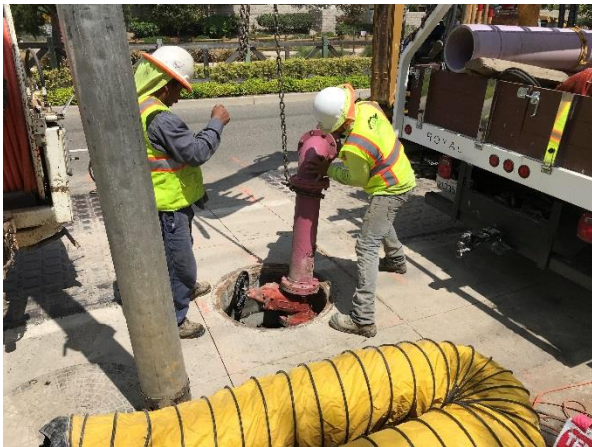
Crews Remove Existing Piping for Vault Removal
